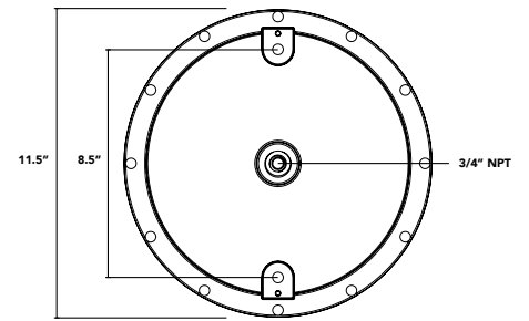
Ceiling Mounting Plate
